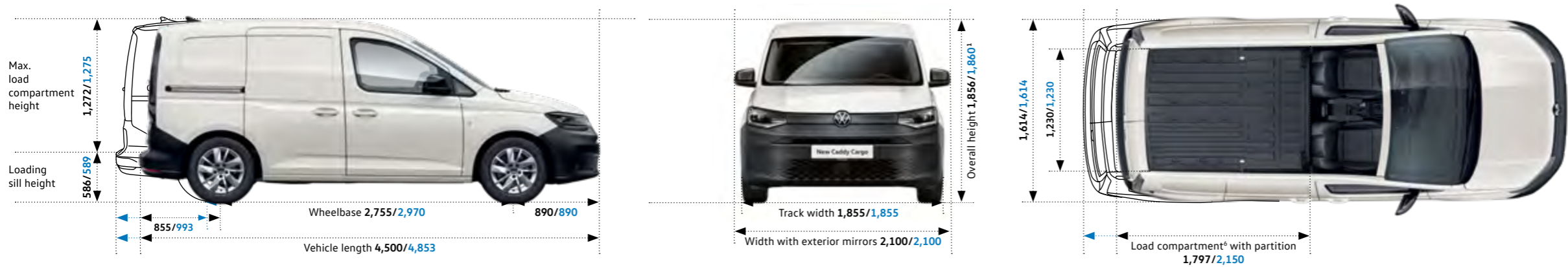
Wider Maxi sliding door (846 x 1,095 mm) for Caddy Cargo Maxi 1
